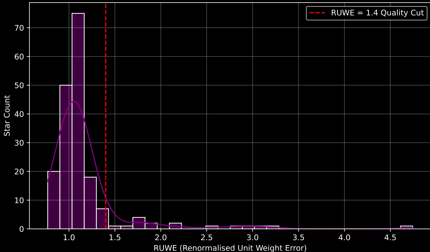
GAPOGEE DR17 Field [CVZTILE_091+35_btx] RUWE Distribution (n= 186)
