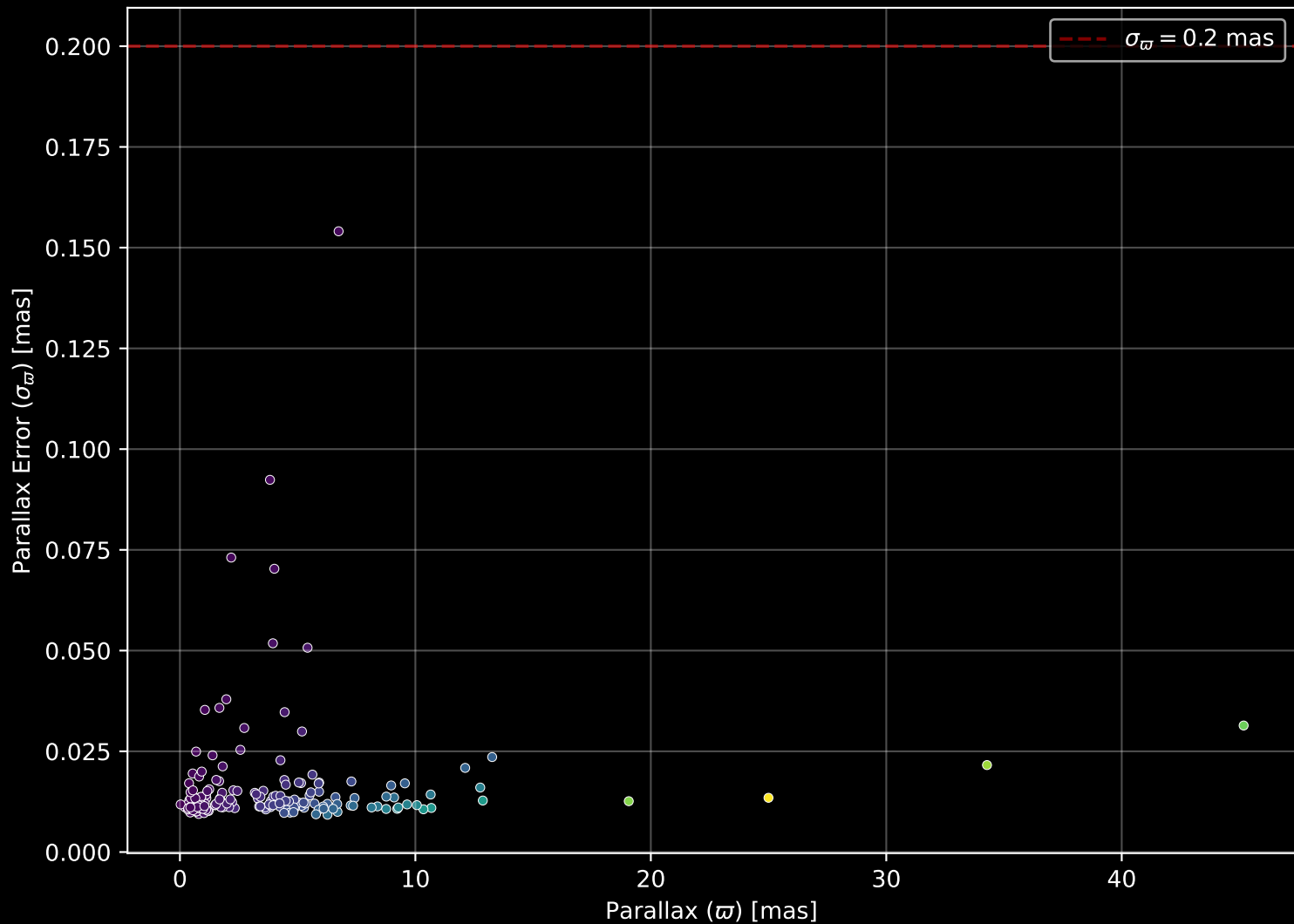
APOGEE DR17 Field: [CVZTILE_091+35_btx] Parallax Quality (n= 189)
