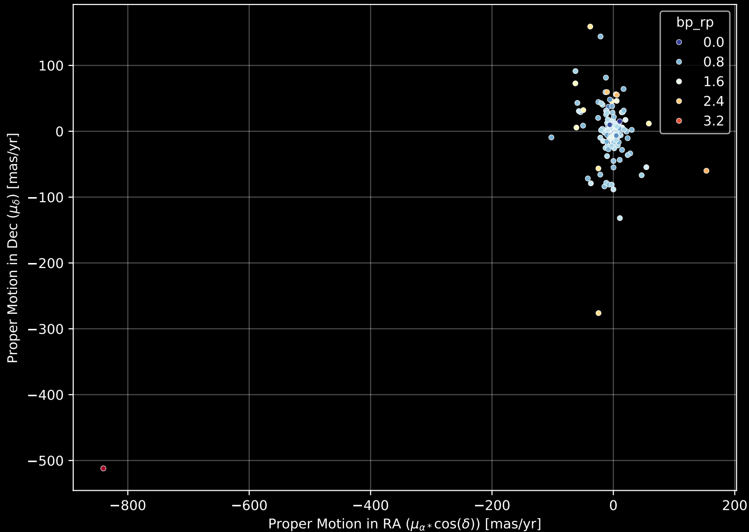
APOGEE DR17 Field: [CVZTILE_091+35_btx] Proper Motion Diagram (n= 189)
