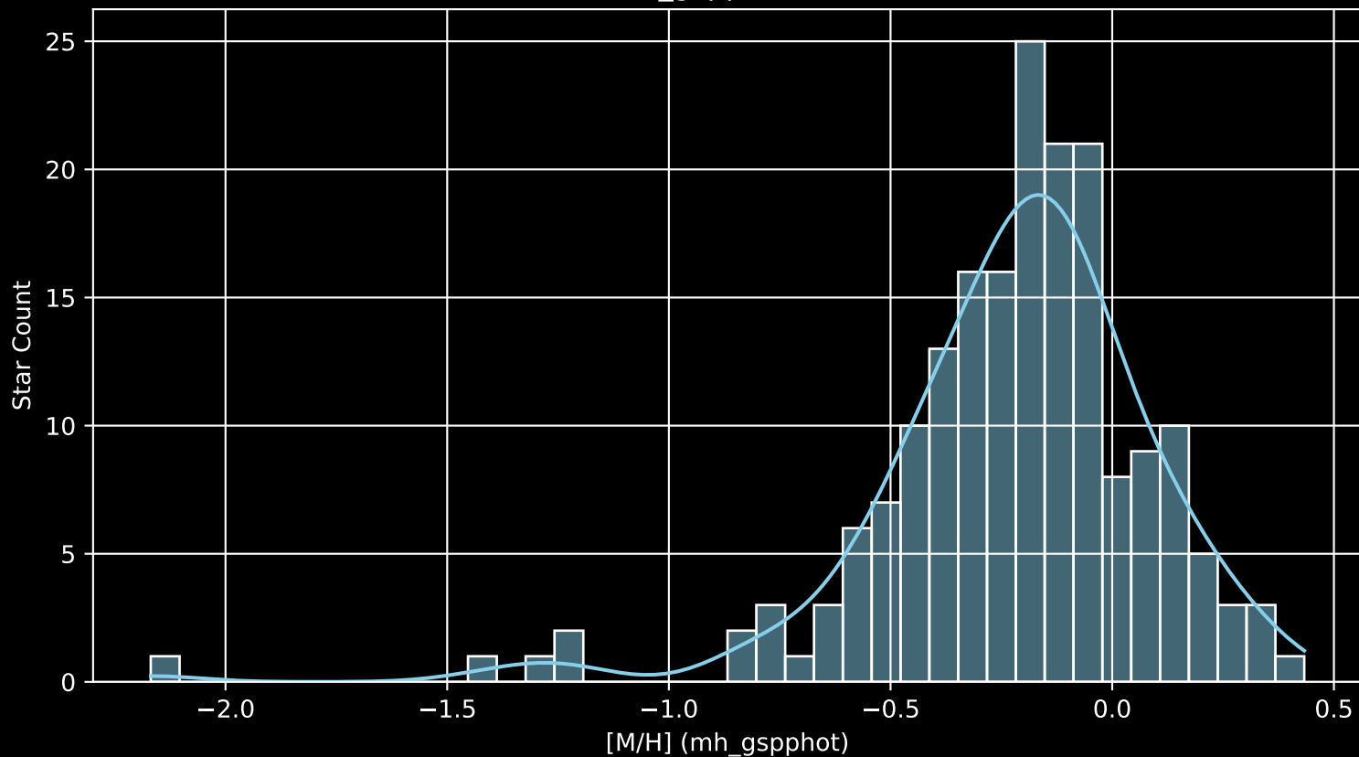
APOGEE DR17 Field: [CVZTILE_091+35_btx [M/H] (mh_gspphot) (n= 188)
