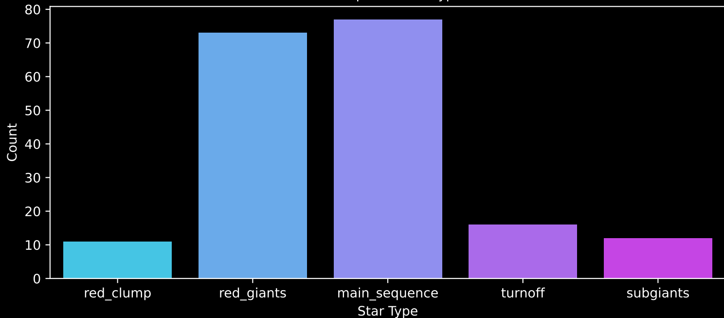
APOGEE DR17 Field: [CVZTILE_091+35_btx] Count plot of Star Type
